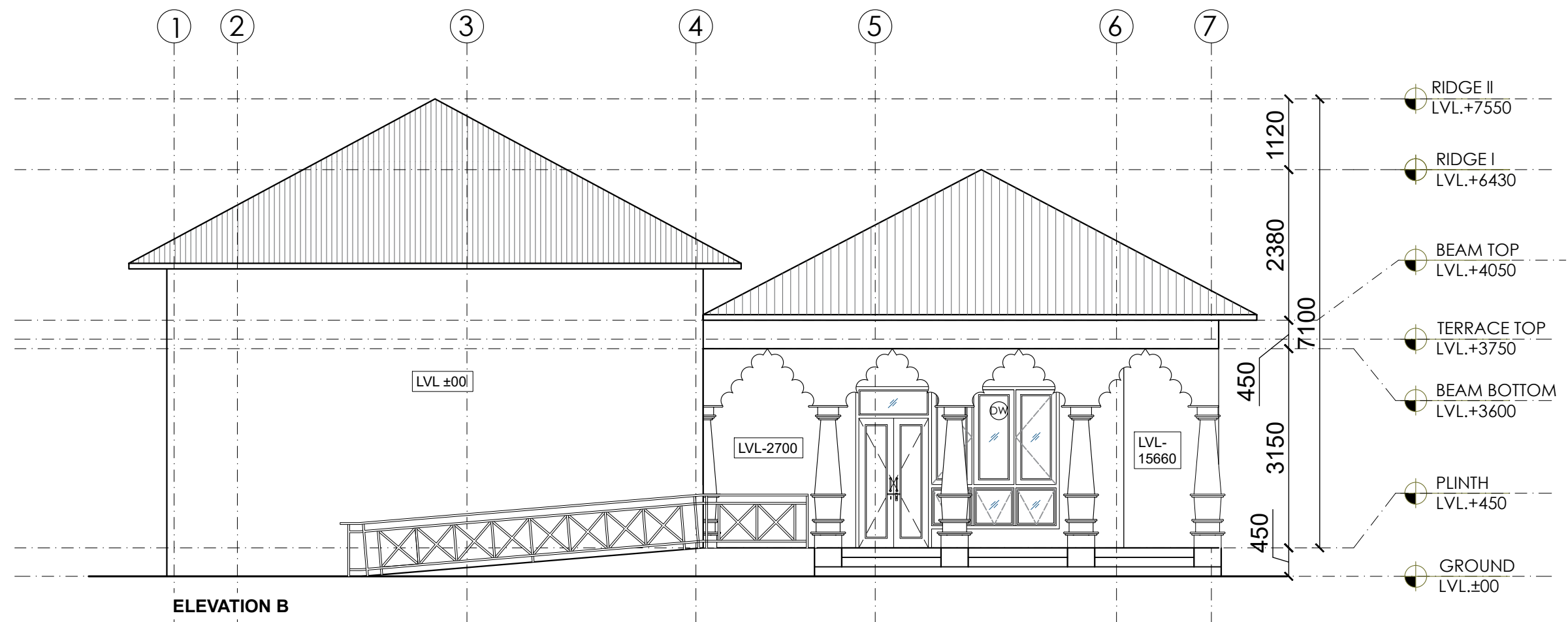
WORKSHOP BUILDING ELEVATIONS
